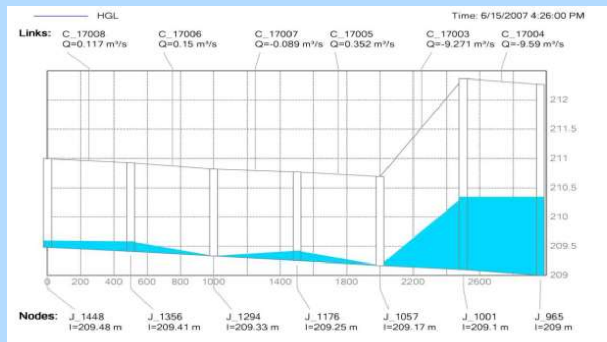
Scenario 5: After the application of storage junctions
