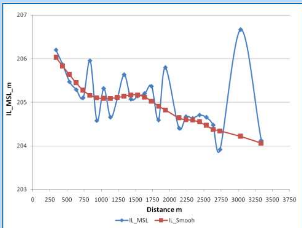
Figure 2.5-2: Illustration of smoothing of Invert Levels
