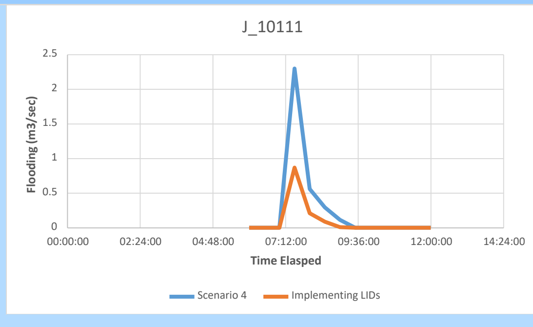
Figure 3.2-25: Graph reflecting the change in Flood volume for J_10111
