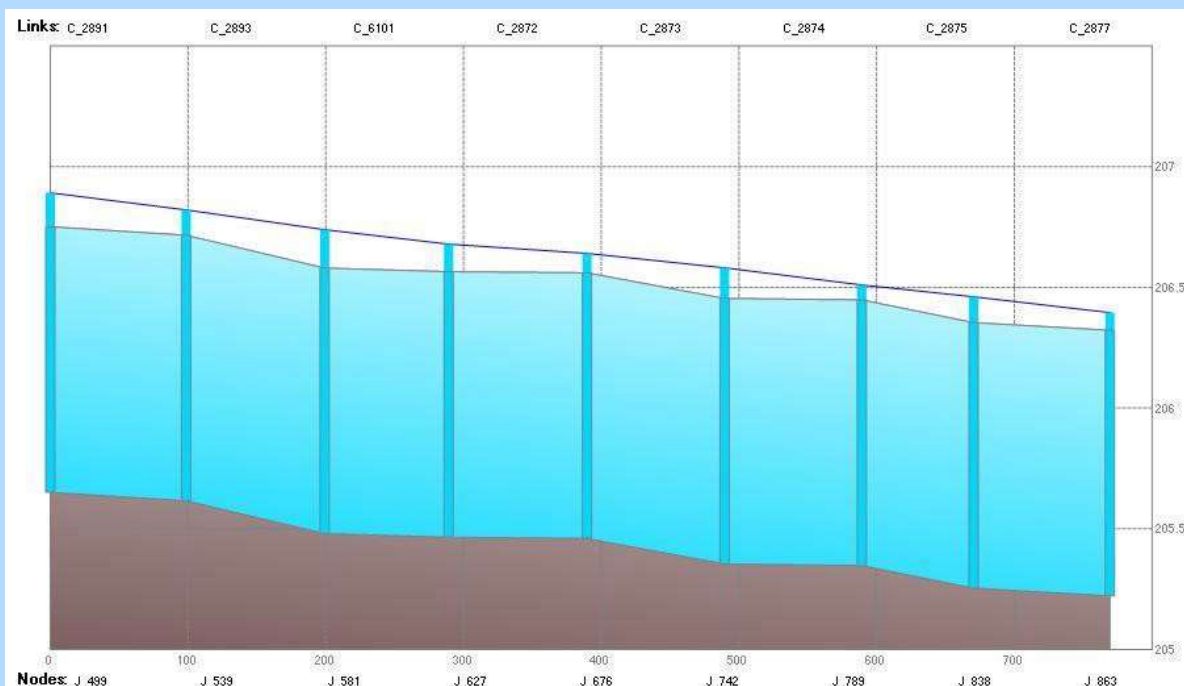
Scenario2: Before inclusion of water body in basin
