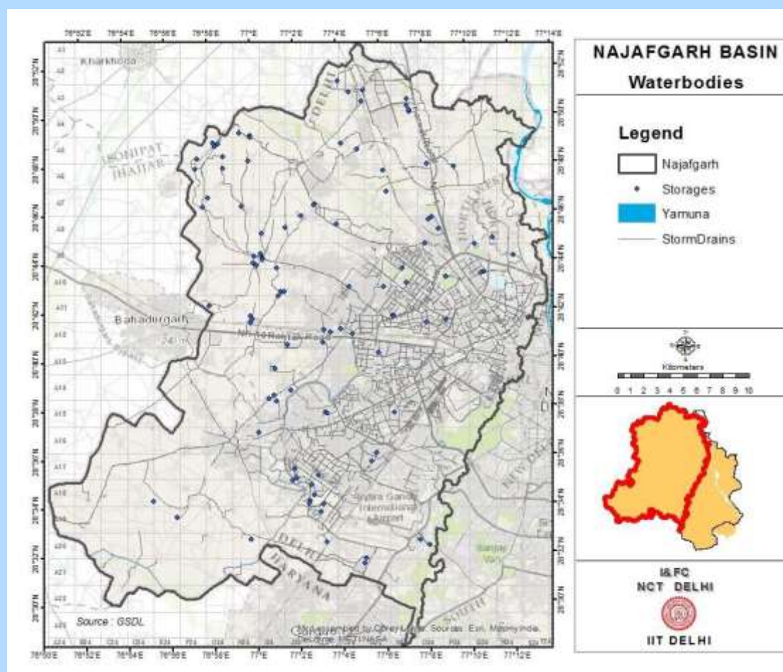
Figure 3.3-11: Water bodies connected to junction to divert the excess water
