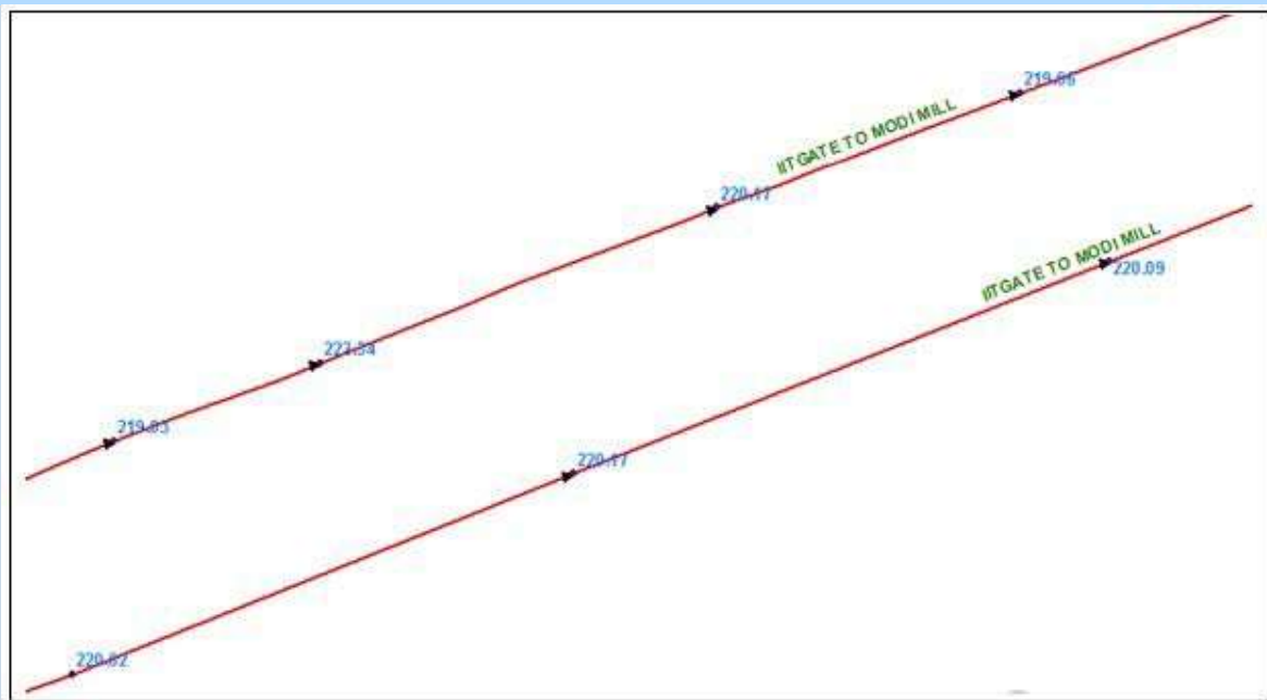
Figure 3.2-10: Direction of flow indicated against the Invert Level slope
