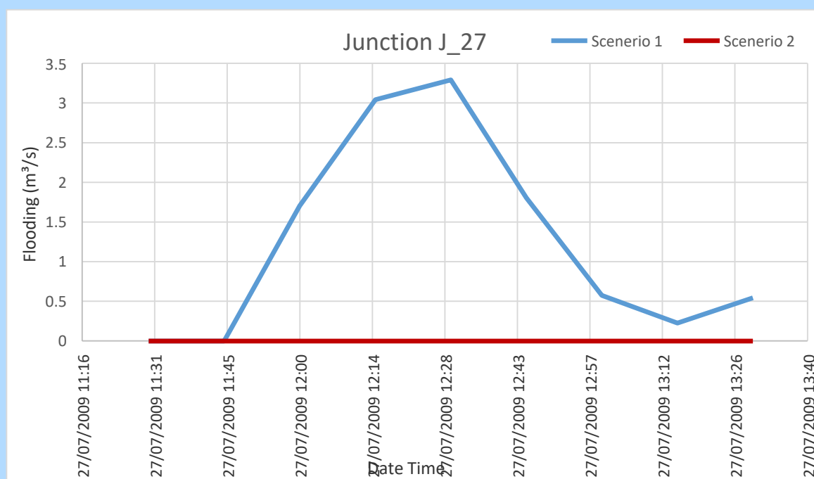
Figure 3.2-13: Comparison between the flood volume at a sample junction after simulation of scenario 1 and scenario 2
