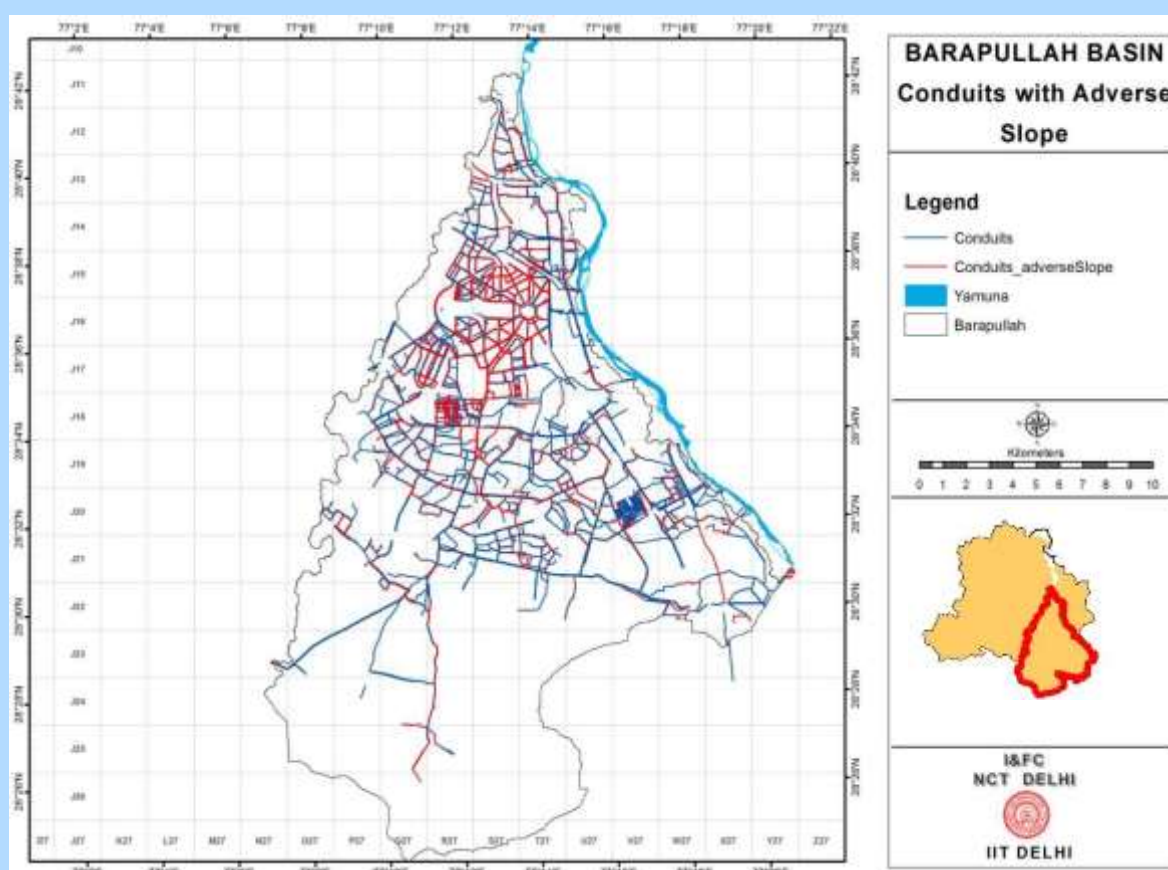
Figure 3.2-11: Barapullah basin showing conduits with negative slope
