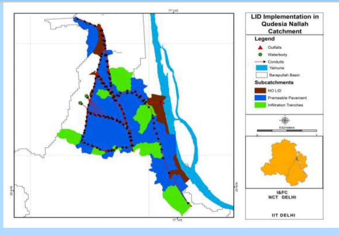
Figure 3.2-24: LID Implementation in Qudesia Nallah Catchment
