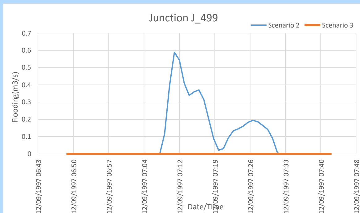
Figure 3.1-15: Comparison between the flood volume at a sample junction after simulation of scenario 2 and scenario 3
