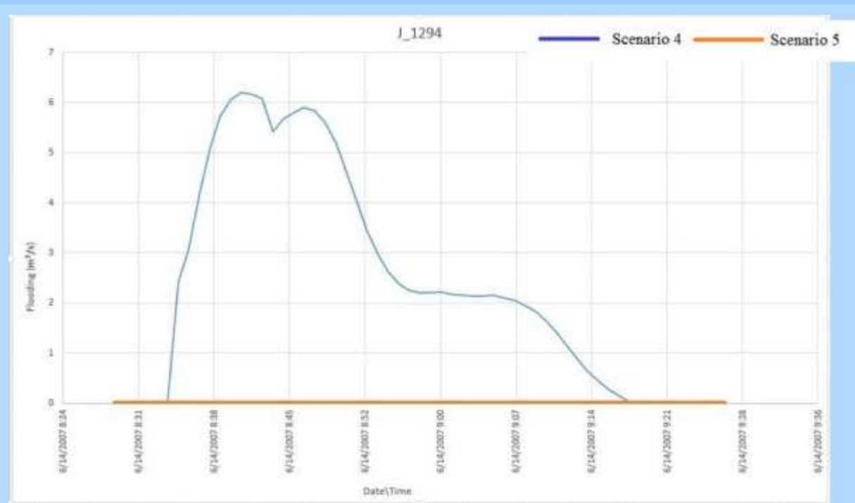
Figure 3.3 19: Comparison between the flood volume at a sample junction after simulation of Scenario 4 and Scenario 5
