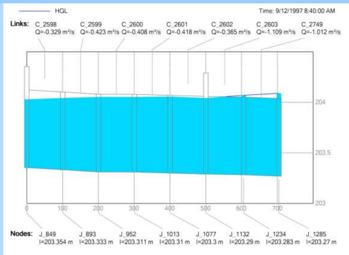
Figure 3.1-20: Comparison of water profile in the segment of the drain after scenario 4 and 5
