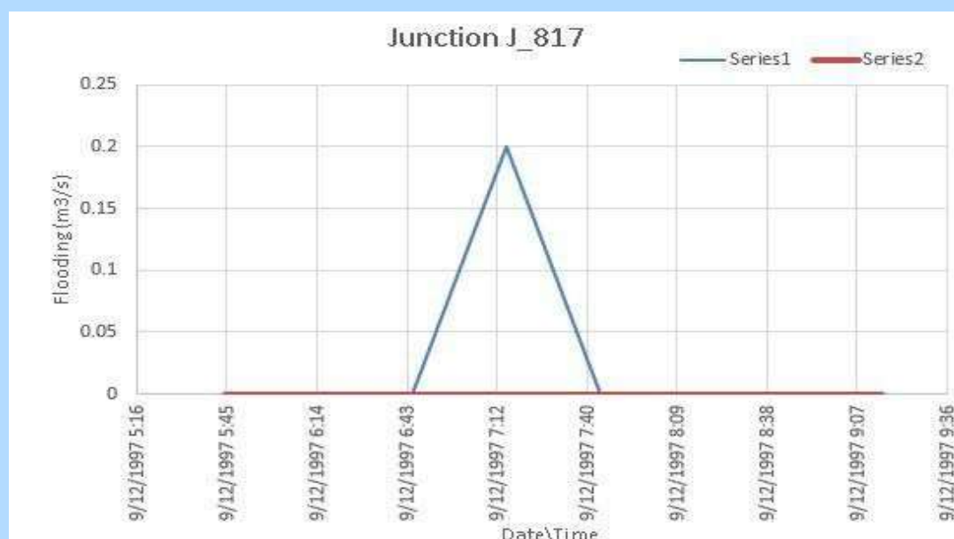
Figure 3.1-12: Comparison between the flood volume at a sample junction after simulation of scenario 1 and scenario2
