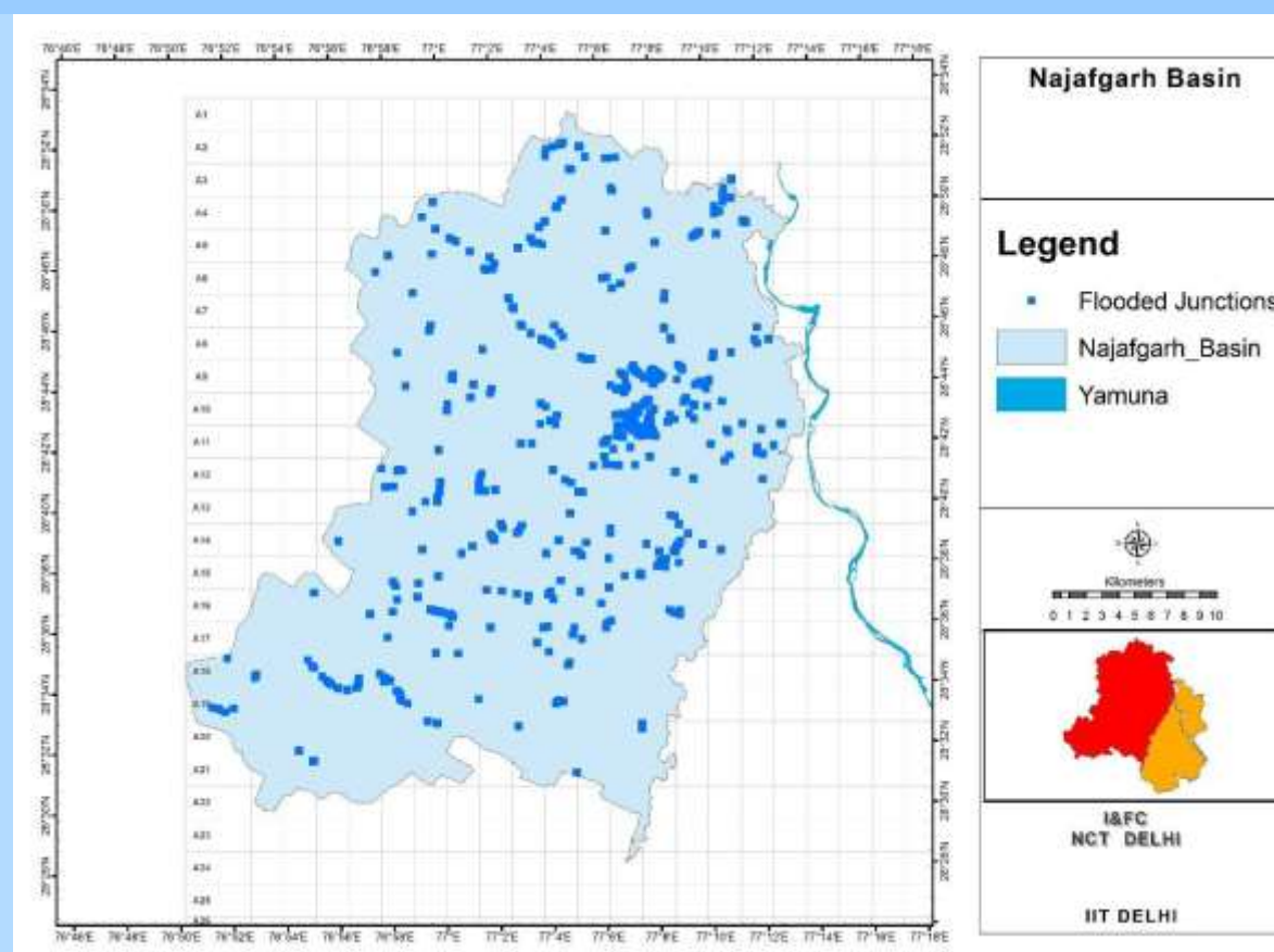
Figure 3.3-17: Flooded junctions were transferred into Storages
