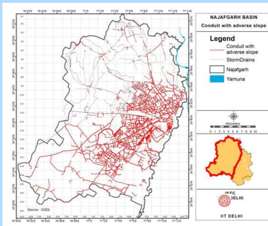
Figure 3.3-8: Conduits with adverse slope in Najafgarh basin
