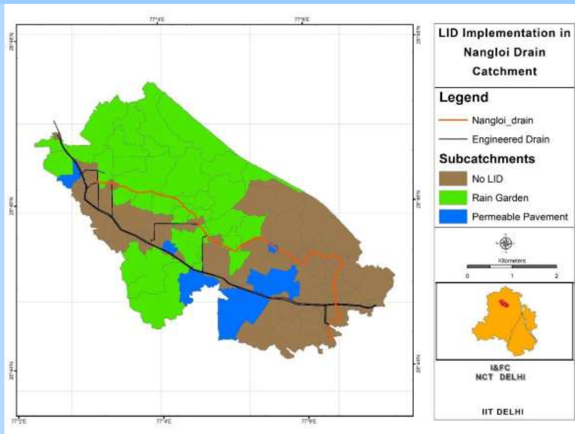
Figure 3.3-20: LID Implementation in Nangloi Drain Catchment
